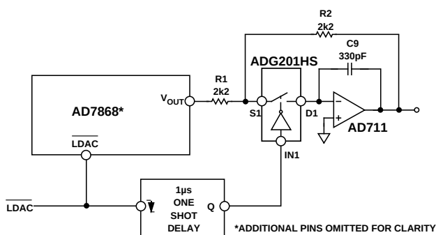
Figure 13. DAC Sample-and-Hold Circuit
