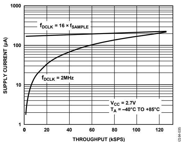
Figure 35. Supply Current vs. Throughput ( \mu A )
