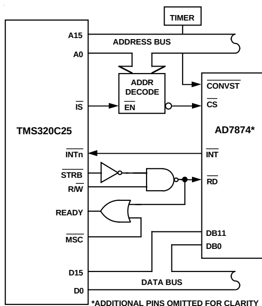
Figure 14. AD7874–TMS320C25 Interface
