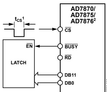
Figure 30. Stand-Alone Operation
