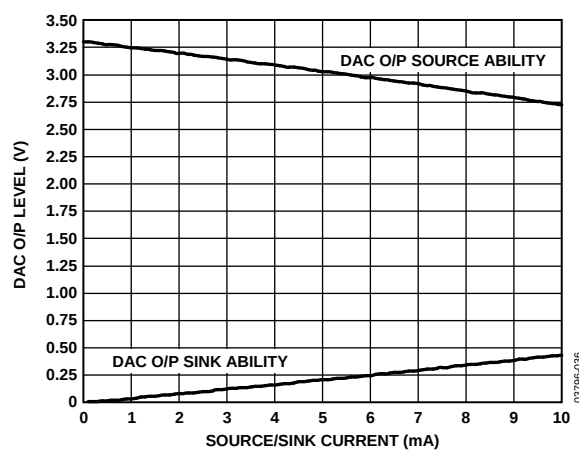
Figure 23. DAC Source and Sink Current Capability
