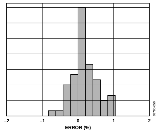
Figure 26. Typical Accuracy for Battery Channel ( 25^{\circ}C )
