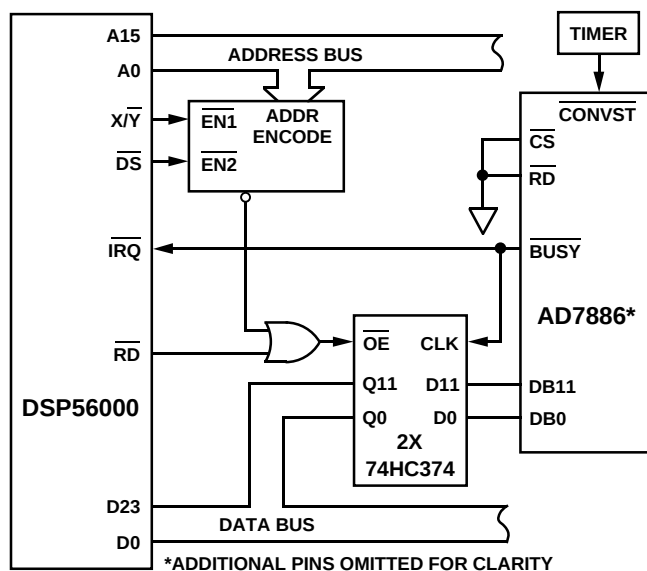
Figure 19. AD7886-DSP56000 Interface
