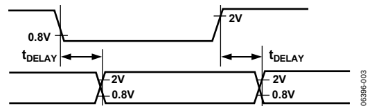
Figure 3. Voltage Reference Levels for Timing
