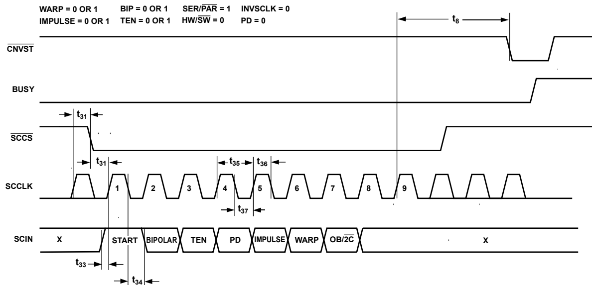
Figure 45. Serial Configuration Port Timing
