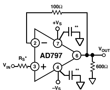
Figure 22. Follower Connection
