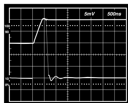
Figure 26. 16-Bit Settling Time Negative Input Pulse
