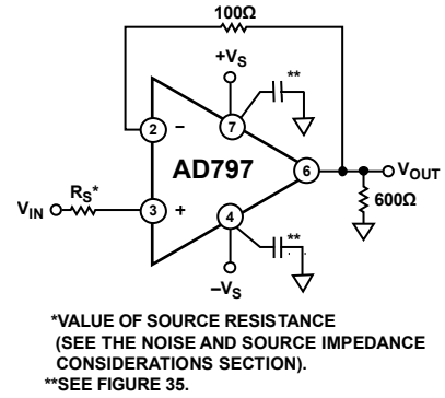
Figure 24. Follower Connection
