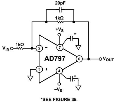
Figure 21. Inverter Connection
