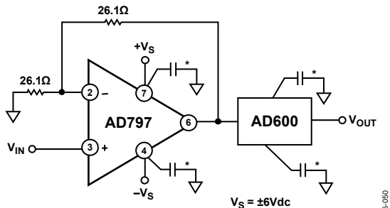
Figure 50. An Ultrasound Preamp Circuit
