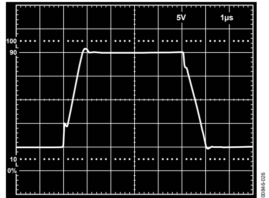
Figure 25. Follower Large-Signal Pulse Response
