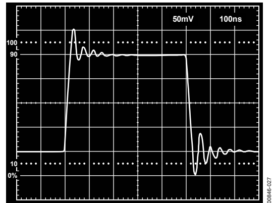
Figure 26. Follower Small-Signal Pulse Response
