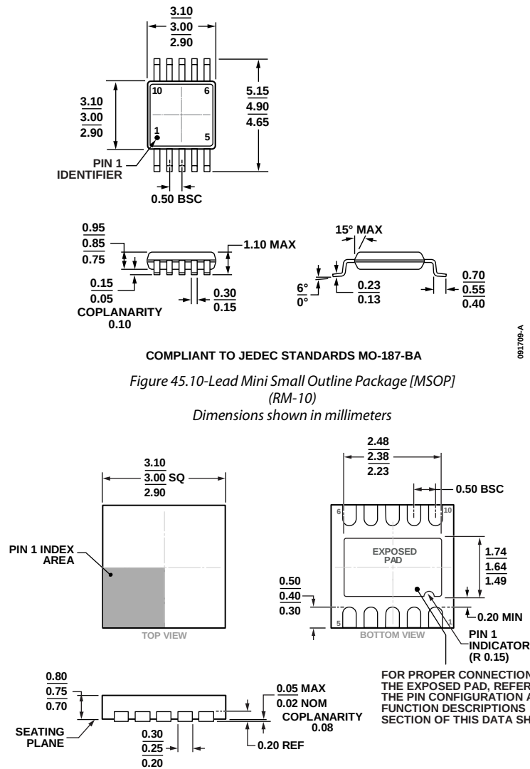
Figure 46. 10-Lead Lead Frame Chip Scale Package [LFCSP_WD] 3 mm x 3 mm Body, Very Very Thin, Dual Lead (CP-10-9)
