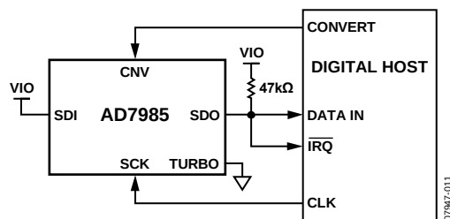
Figure 28. \overline{\text{CS}} Mode, 3-Wire with Busy Indicator Connection Diagram ( \overline{\text{SDI}} High)
