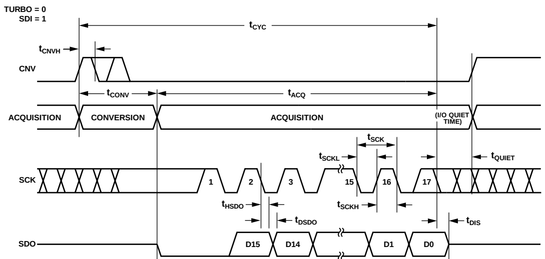
Figure 29. \overline{\text{CS}} Mode, 3-Wire with Busy Indicator Serial Interface Timing ( \overline{\text{SDI}} High)
