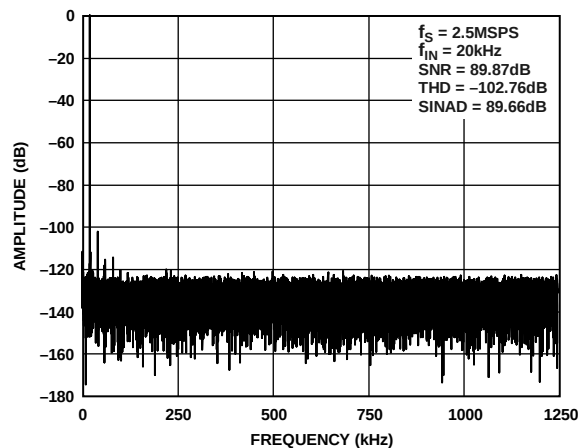
Figure 11. FFT Plot (External Reference)
