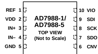
Figure 5. 10-Lead LFCSP (QFN) Pin Configuration
