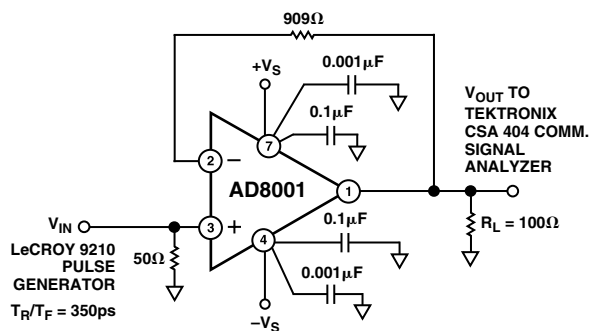
TPC 5. Test Circuit, Gain = +1
