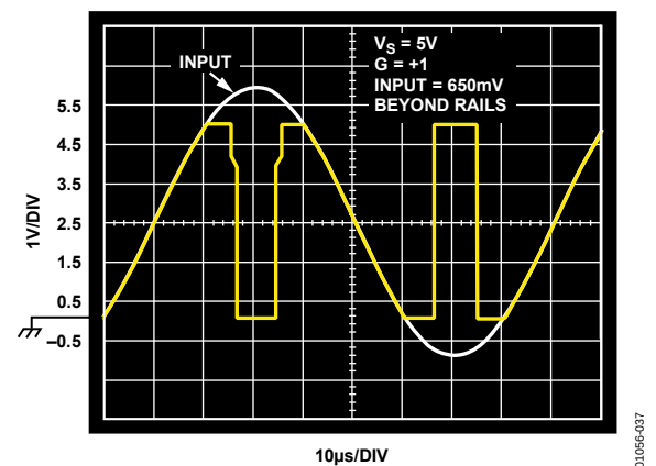
Figure 37. Output Voltage Phase Reversal Behavior
