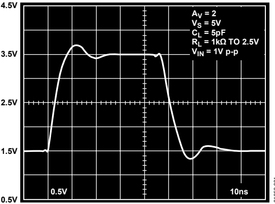
Figure 31. 1 V Pulse Response, V_S = 5\text{ V}
