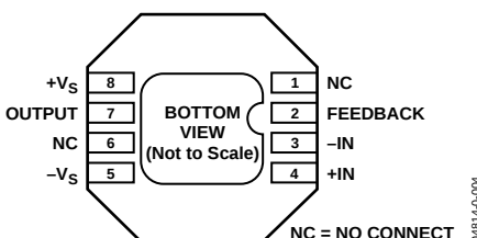
Figure 6. 8-Lead LFCSP Pin Configuration
