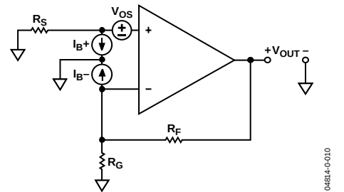
Figure 65. Amplifier DC Errors
