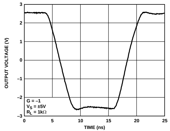
Figure 41. Large Signal Transient Response, Inverting
