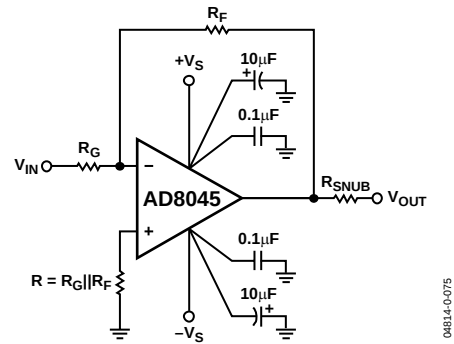
Figure 62. Inverting Configuration
