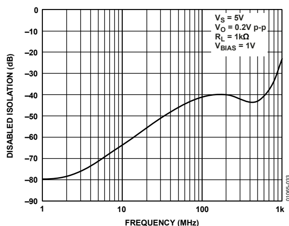
Figure 33. AD8063 Disabled Output Isolation Frequency Response
