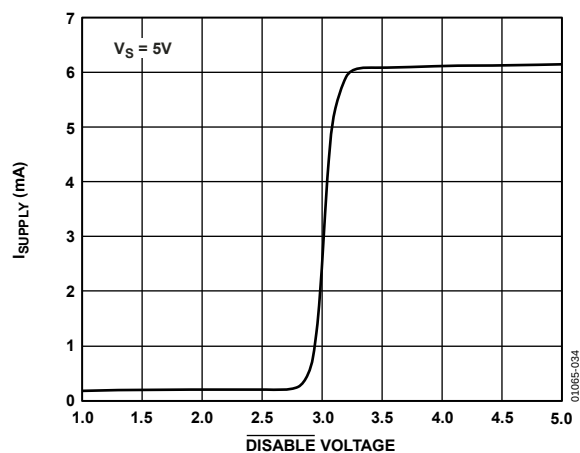
Figure 34. AD8063 \overline{DISABLE} Voltage vs. Supply Current
