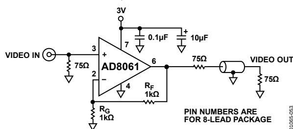
Figure 53. Single 3 V Sync Stripper Using AD8061
