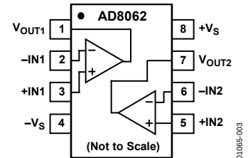
Figure 2. 8-Lead SOIC (R)/MSOP (RM)
