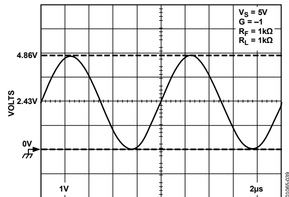
Figure 39. Output Swing
