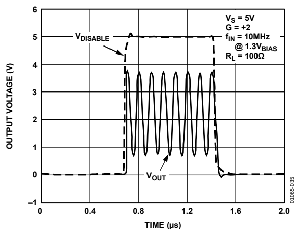
Figure 35. AD8063 \overline{DISABLE} Function, Voltage = 0 V to 5 V
