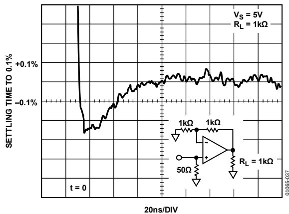
Figure 37. Output Settling Time to 0.1%
