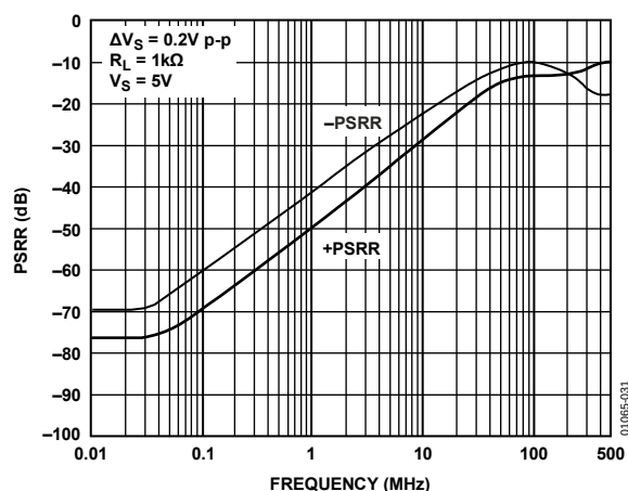
Figure 31. \pm PSRR vs. Frequency Delta
