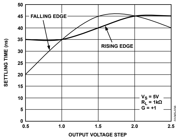
Figure 38. Settling Time vs. V_{OUT}
