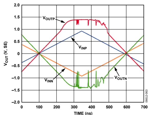
Figure 63. AD8105 Overdrive Recovery, Single-Ended
