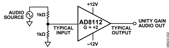
Figure 44. Input Divide Circuit
