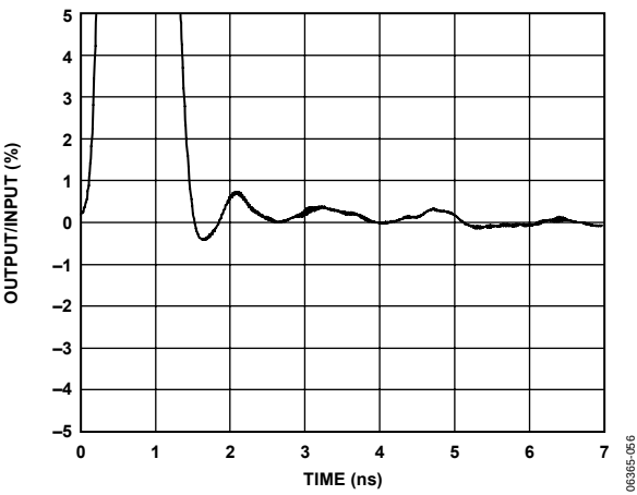
Figure 61. AD8117 Settling Time (Zoom)
