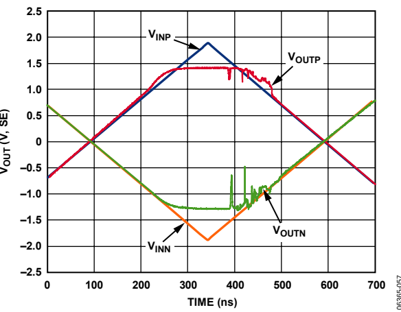
Figure 62. AD8117 Overdrive Recovery, Single-Ended
