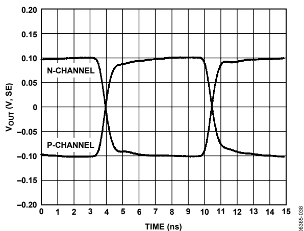
Figure 43. AD8117 Small Signal Pulse Response, Single-Ended, 200 mV p-p
