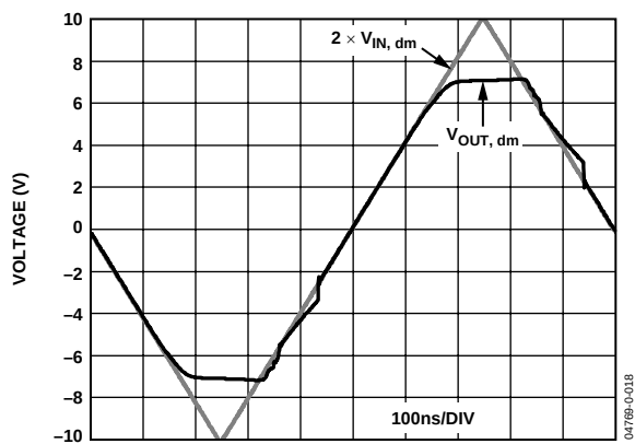
Figure 14. Overdrive Recovery
