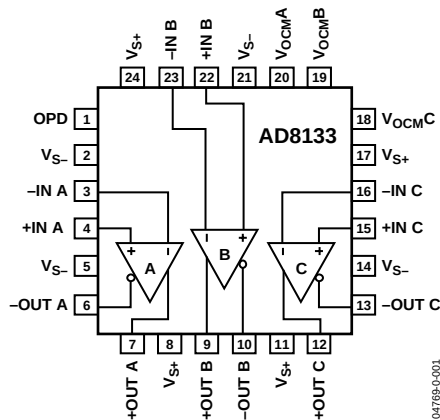
Figure 4. 24-Lead LFCSP
