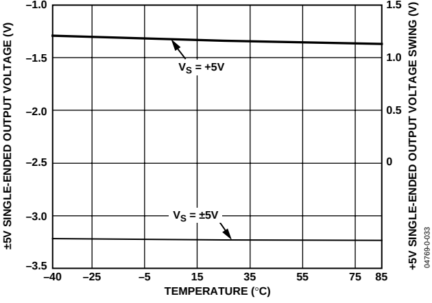
Figure 33. Negative Output Saturation Voltage vs. Temperature
