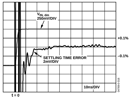
Figure 17. Settling Time (0.1%)
