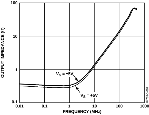
Figure 32. Single-Ended Output Impedance Magnitude vs. Frequency
