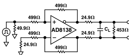
TPC 23. Test Circuit for Cap Load Drive
