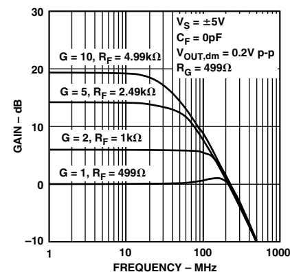
TPC 6. Small Signal Frequency Response for Various Gains
