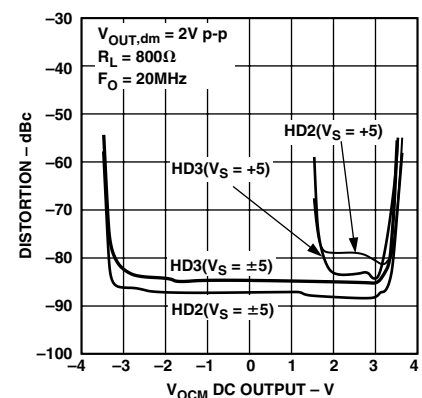
TPC 9. Harmonic Distortion vs. V_{OCM}
