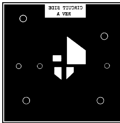
Figure 31. AD8170 Board Layout (Solder Side)
