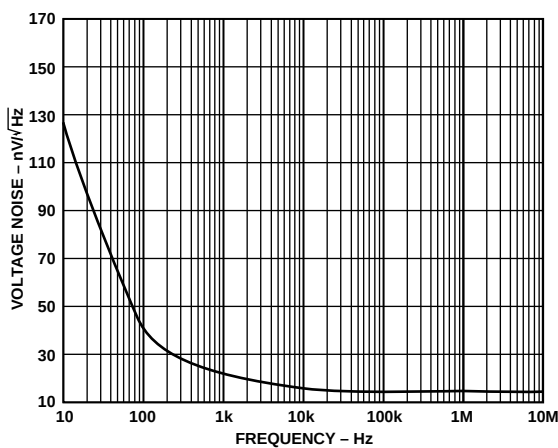
Figure 26. AD8185 RTI Voltage Noise vs. Frequency
