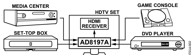
Figure 2. Typical HDTV Application
