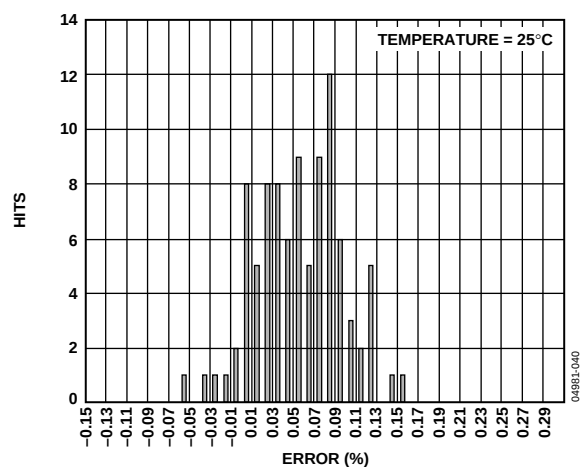
Figure 22. MSOP Gain Accuracy, Temperature = 25°C
