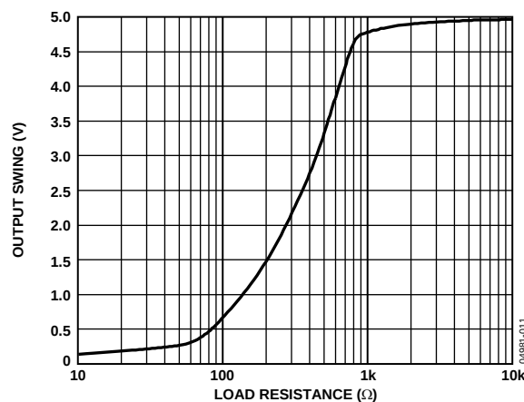
Figure 11. Output Swing vs. Load Resistance
