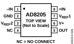
Figure 3. Pin Configuration
