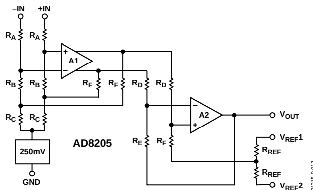
Figure 13. Simplified Schematic
