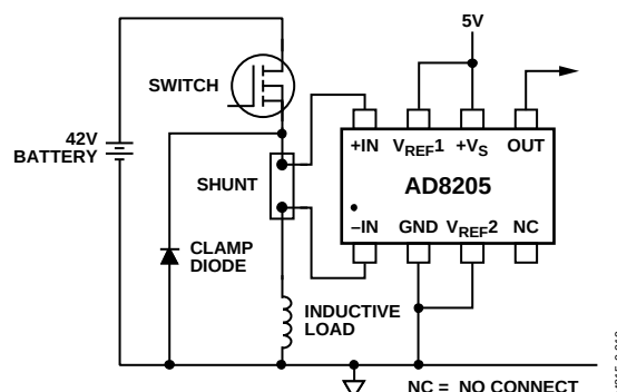
Figure 20. High-Side Switch
