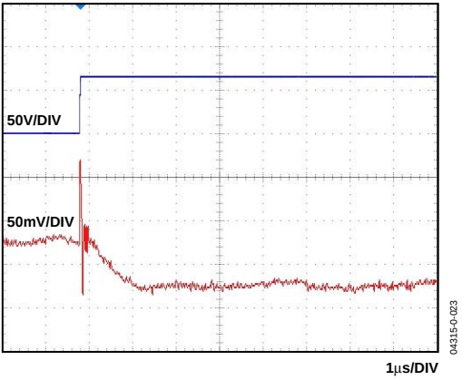
Figure 12. Common-Mode Response
