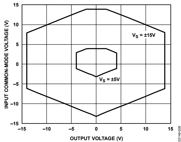
Figure 8. Input Common-Mode Range vs. Output Voltage, G = 10
