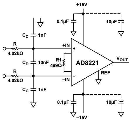
Figure 48. RFI Suppression
