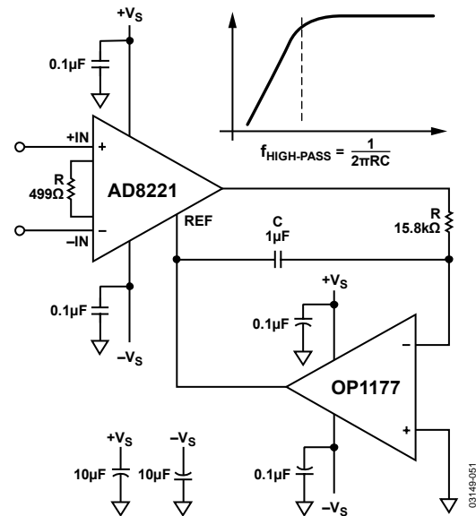
Figure 51. AC-Coupled Circuit
