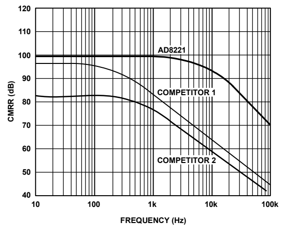
Figure 2. Typical CMRR vs. Frequency for G = 1
