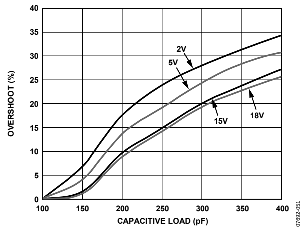
Figure 32. Small-Signal Overshoot vs. Capacitive Load, R_L \geq 2k\Omega
