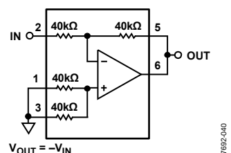
Figure 40. Inverting Amplifier, Gain = -1
