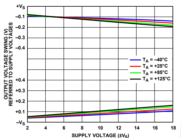
Figure 16. Output Voltage Swing vs. Supply Voltage and Temperature, R_L = 10 k \Omega
