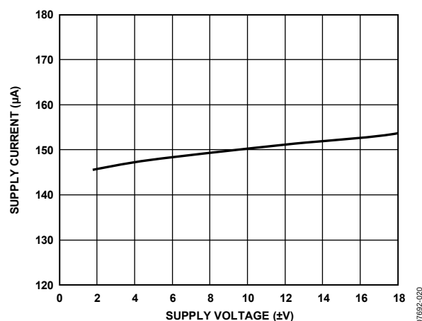
Figure 20. Supply Current vs. Dual Supply Voltage, V_{IN} = 0\text{ V}
