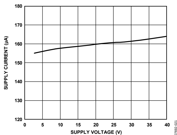
Figure 21. Supply Current vs. Single-Supply Voltage, V_{IN} = 0\text{ V} , V_{REF} = 0\text{ V}
