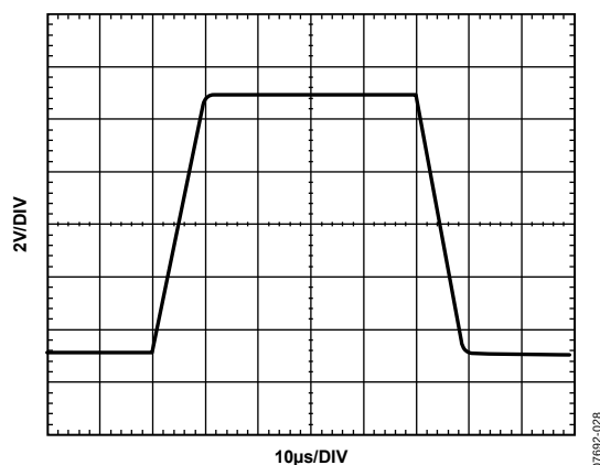
Figure 28. Large-Signal Step Response
