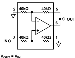
Figure 41. Noninverting Amplifier, Gain = 1
