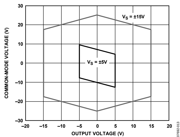
Figure 13. Input Common-Mode Voltage vs. Output Voltage, \pm 15 V and \pm 5 V Supplies
