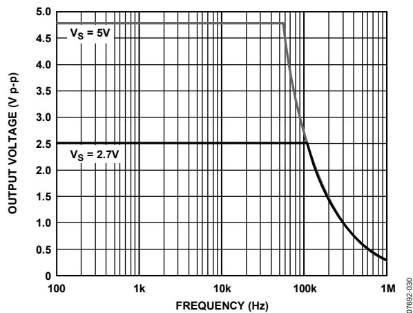
Figure 30. Maximum Output Voltage vs. Frequency, V_S = 5V, 2.7V
