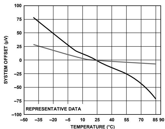
Figure 8. System Offset vs. Temperature, Normalized at 25^\circ\text{C}
