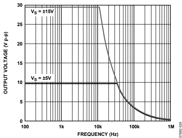
Figure 29. Maximum Output Voltage vs. Frequency, V_S = \pm 15V, \pm 5V
