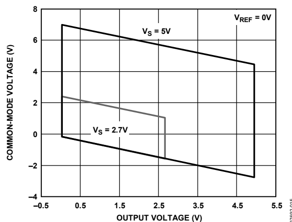
Figure 15. Input Common-Mode Voltage vs. Output Voltage, 5 V and 2.7 V Supplies, V_{REF} = 0 V
