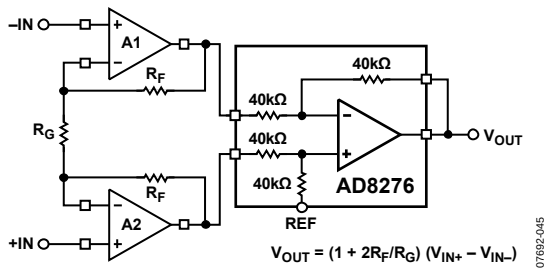
Figure 44. Low Power Precision Instrumentation Amplifier
