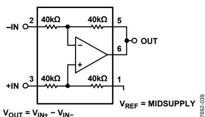
Figure 39. Difference Amplifier, Gain = 1, Referenced to Midsupply
