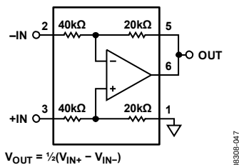
Figure 48. Difference Amplifier, Gain = 1/2
