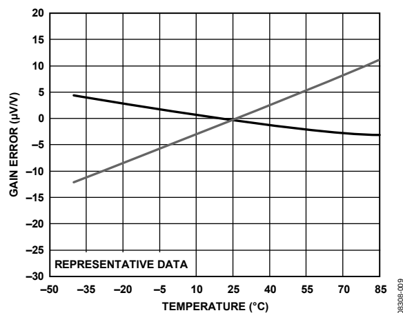
Figure 9. Gain Error vs. Temperature, Normalized at 25^\circ\text{C} , G = \frac{1}{2}
