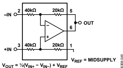
Figure 50. Difference Amplifier, Gain = 1/2, Referenced to Midsupply
