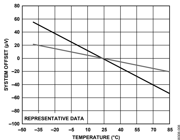
Figure 8. System Offset vs. Temperature, Normalized at 25^\circ\text{C} , G = \frac{1}{2}
