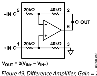
Figure 49. Difference Amplifier, Gain = 2
