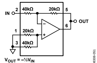
Figure 52. Inverting Amplifier, Gain = -1/2
