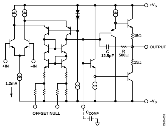
Figure 35. Simplified Schematic
