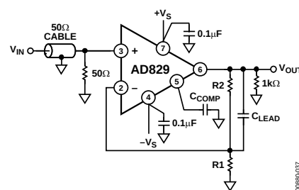
Figure 37. Noninverting Amplifier Connection Using External Shunt Compensation
