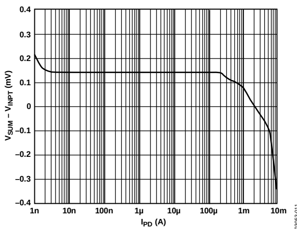
Figure 11. V_{INPT} - V_{SUM} vs. I_{PD}
