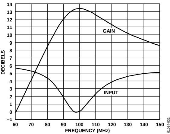
Figure 32. Response of 100 MHz Matching Network
