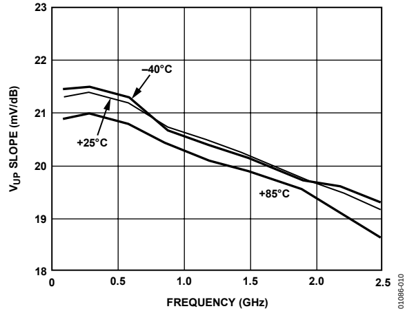
Figure 10. Slope vs. Frequency; -40°C, +25°C, and +85°C
