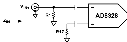
Figure 23. Single-Ended Circuit
