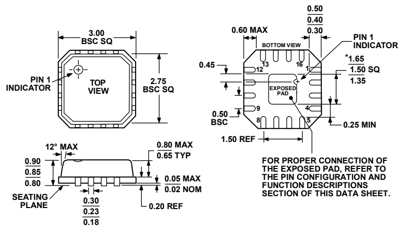
*COMPLIANT TO JEDEC STANDARDS MO-220-VEED-2 EXCEPT FOR EXPOSED PAD DIMENSION. Figure 63. 16-Lead Lead Frame Chip Scale Package [LFCSP_VQ] 3 mm x 3 mm Body, Very Thin Quad (CP-16-3) Dimensions in millimeters
