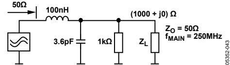
Figure 42. Matching Circuit
