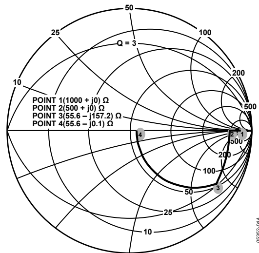
Figure 43. LC Matching Example
