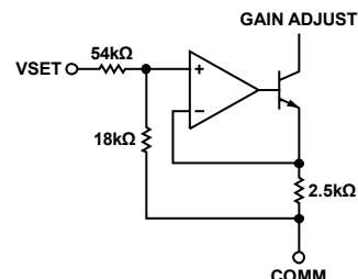
Figure 40. VSET Interface Simplified Schematic
