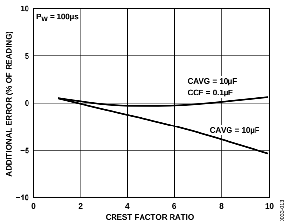
Figure 14. Crest Factor Error vs. Crest Factor for CAVG and CAVG and CCF Capacitor Combinations
