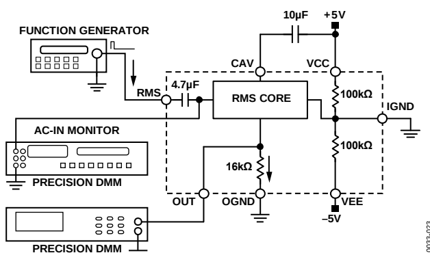
Figure 23. Crest Factor Test Circuit
