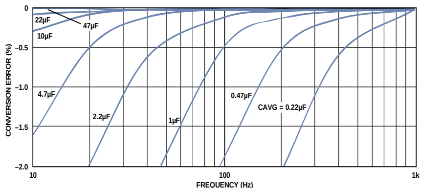
Figure 28. Conversion Error vs. Frequency for Various Values of CAVG
