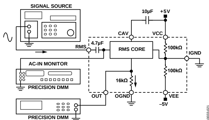
Figure 21. Core Response Test Circuit Using Dual Supplies
