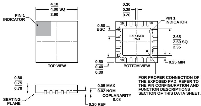
Figure 49. 20-Lead Lead Frame Chip Scale Package [LFCSP_WQ] (CP-20-10)
