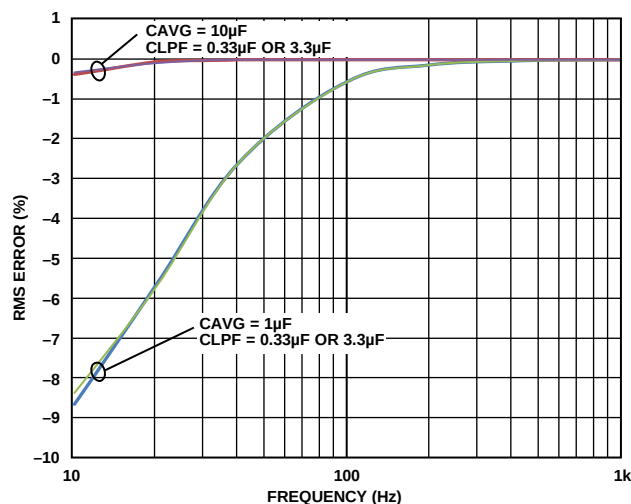
Figure 27. RMS Error vs. Frequency for Two Values of CAVG and CLPF (Note that only CAVG value affects rms error; CLPF has no effect.)
