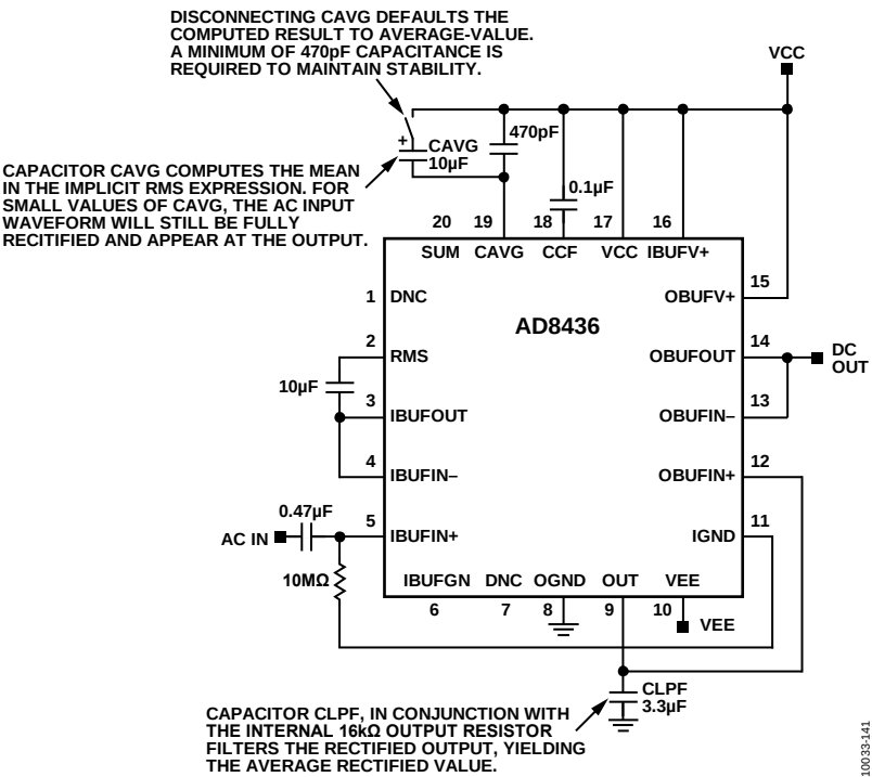
Figure 41. Configuration for Average Rectified Value
