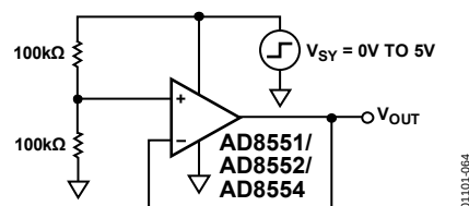
Figure 64. AD855x Test Circuit for Turn-On Time
