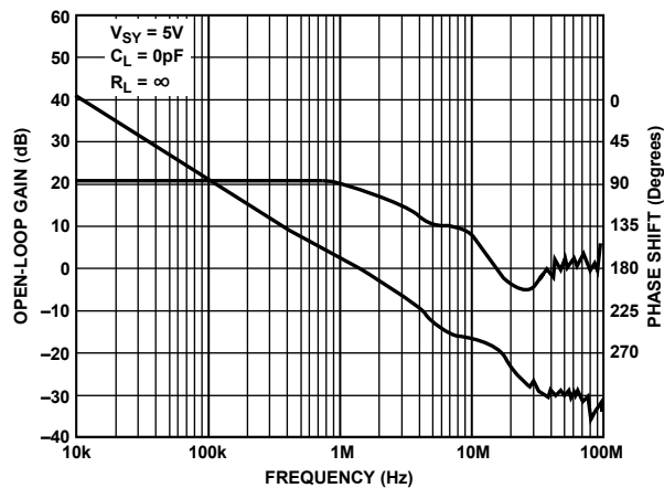
Figure 18. Open-Loop Gain and Phase Shift vs. Frequency at 5 V
