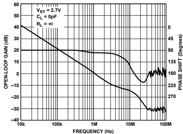
Figure 17. Open-Loop Gain and Phase Shift vs. Frequency at 2.7 V
