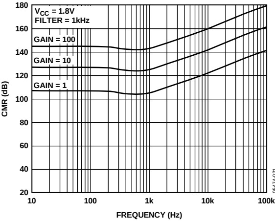
Figure 20. Common-Mode Rejection (CMR) vs. Frequency
