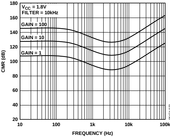
Figure 23. Common-Mode Rejection (CMR) vs. Frequency
