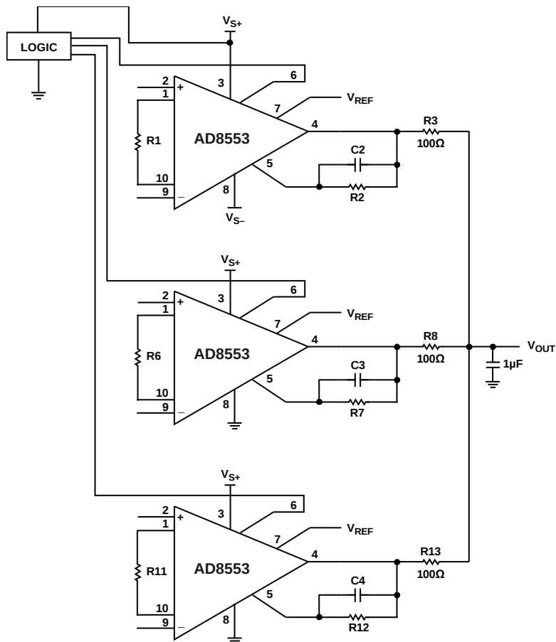
Figure 37. Multiplexed Output
