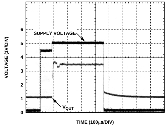
Figure 33. Power-On Response at 125^{\circ}C
