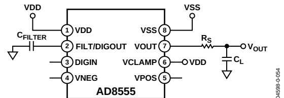
Figure 56. Test Circuit for Driving Capacitive Loads
