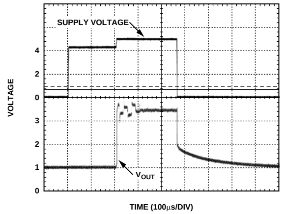
Figure 32. Power-On Response at 25^{\circ}C
