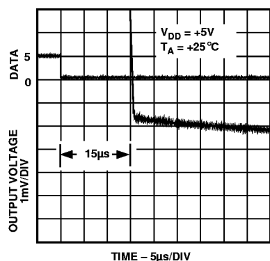
Figure 14. Output Voltage Fall Time Detail
