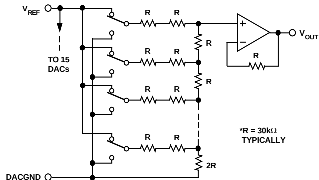
Figure 16. Equivalent Schematic of Analog Channel
