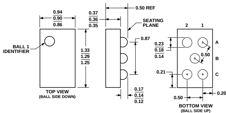
Figure 58. 5-Ball Wafer Level Chip Scale Package [WLCSP] (CB-5-1)
