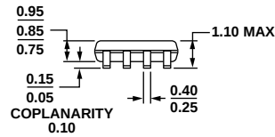
Figure 38. 8-Lead Mini Small Outline Package [MSOP] (RM-8)
