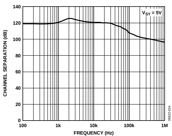
Figure 27. Channel Separation
