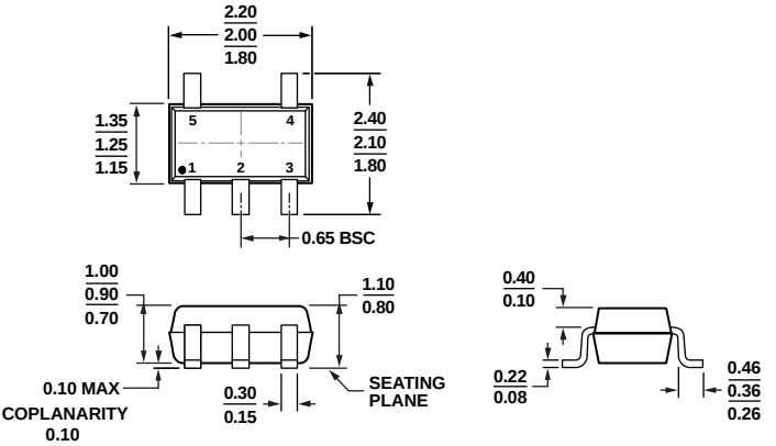
COMPLIANT TO JEDEC STANDARDS MO-203-AA Figure 42. 5-Lead Thin Shrink Small Outline Transistor Package [SC70] (KS-5) Dimensions shown in millimeters
