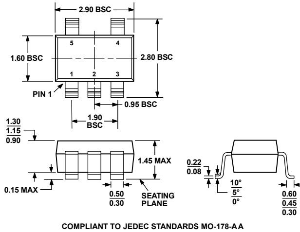
Figure 51. 5-Lead Small Outline Transistor Package [SOT-23] (RJ-5)
