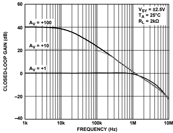
Figure 16. Closed-Loop Gain vs. Frequency
