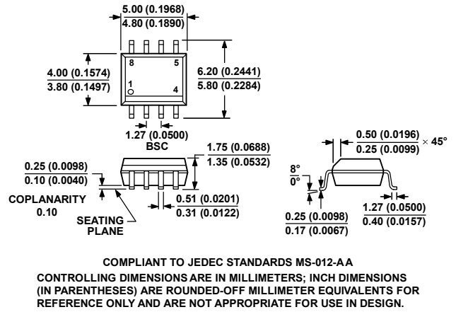
Figure 52. 8-Lead Standard Small Outline Package [SOIC_N] Narrow Body
