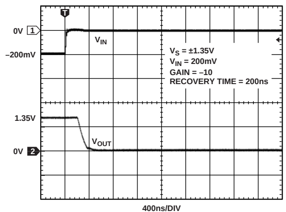
Figure 46. Positive Overload Recovery Time
