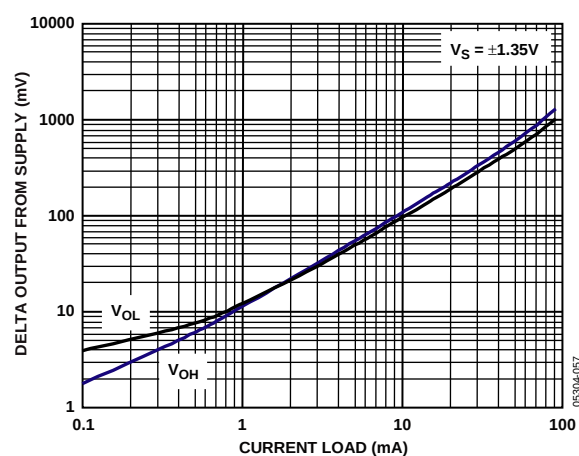
Figure 38. AD8656 Output Swing vs. Current Load
