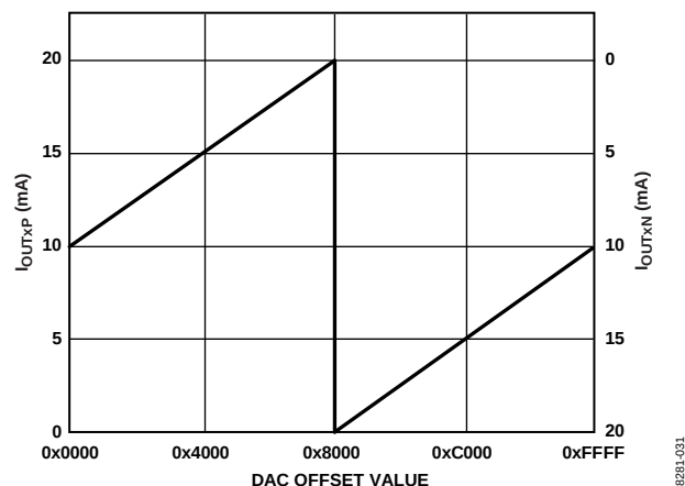
Figure 59. DAC Output Currents vs. DAC Offset Value
