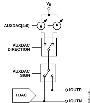
Figure 70. Auxiliary DAC Structure
