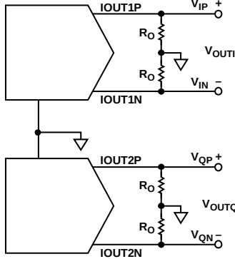
Figure 66. Basic Transmit DAC Output Circuit
