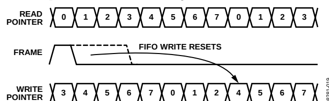
Figure 45. Timing of the FRAME Input vs. Write Pointer Value
