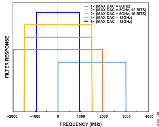
Figure 70. Band Responses of Total Interpolation Rates for 1×, 2×, 4×, and 6× at Each Respective Maximum Achievable DAC Rate and Resolution
