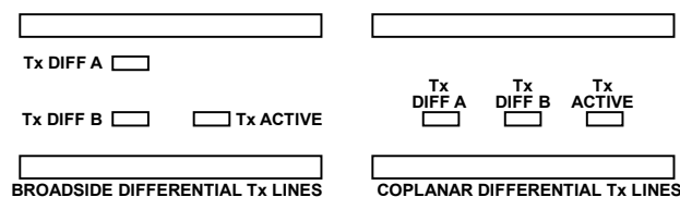
Figure 95. Broadside vs. Coplanar Differential Stripline Routing Techniques
