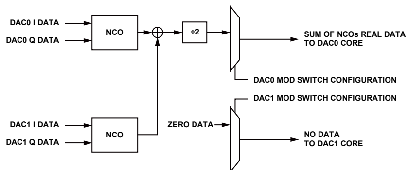
Figure 84. Configuration 3, CMPLX\_MOD\_DIV2\_DISABLE = 0 —DAC0 = I0 + I1 , DAC1 = 0
