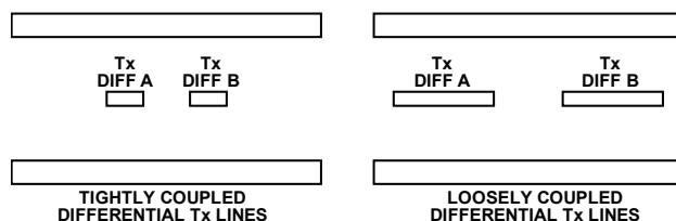
Figure 96. Tightly Coupled vs. Loosely Coupled Differential Traces
